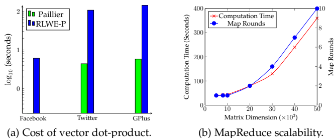
Fig. 5: Cloud-side processing.
